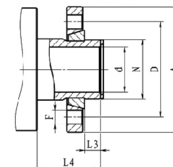
HS-G 双通/固定式内管 DUAL FLOW STATIONARY INTERNAL PIPE
